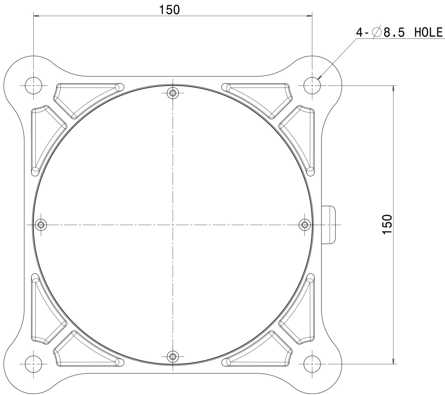
BASE (BOTTOM VIEW) (1:1)
