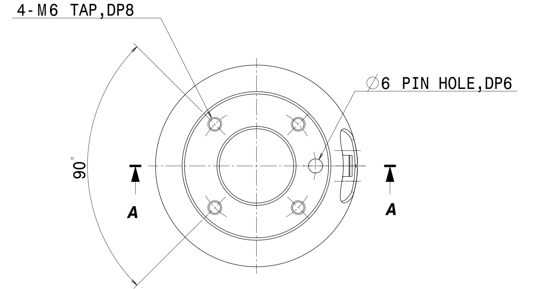
END FLANGE (1:1)
